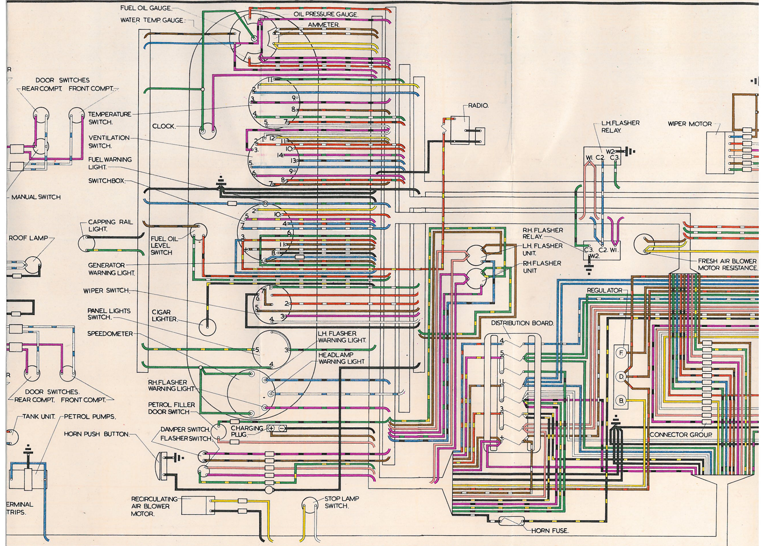
WIRING DIAGRAM RIGHT HAND DRIVE CAR
