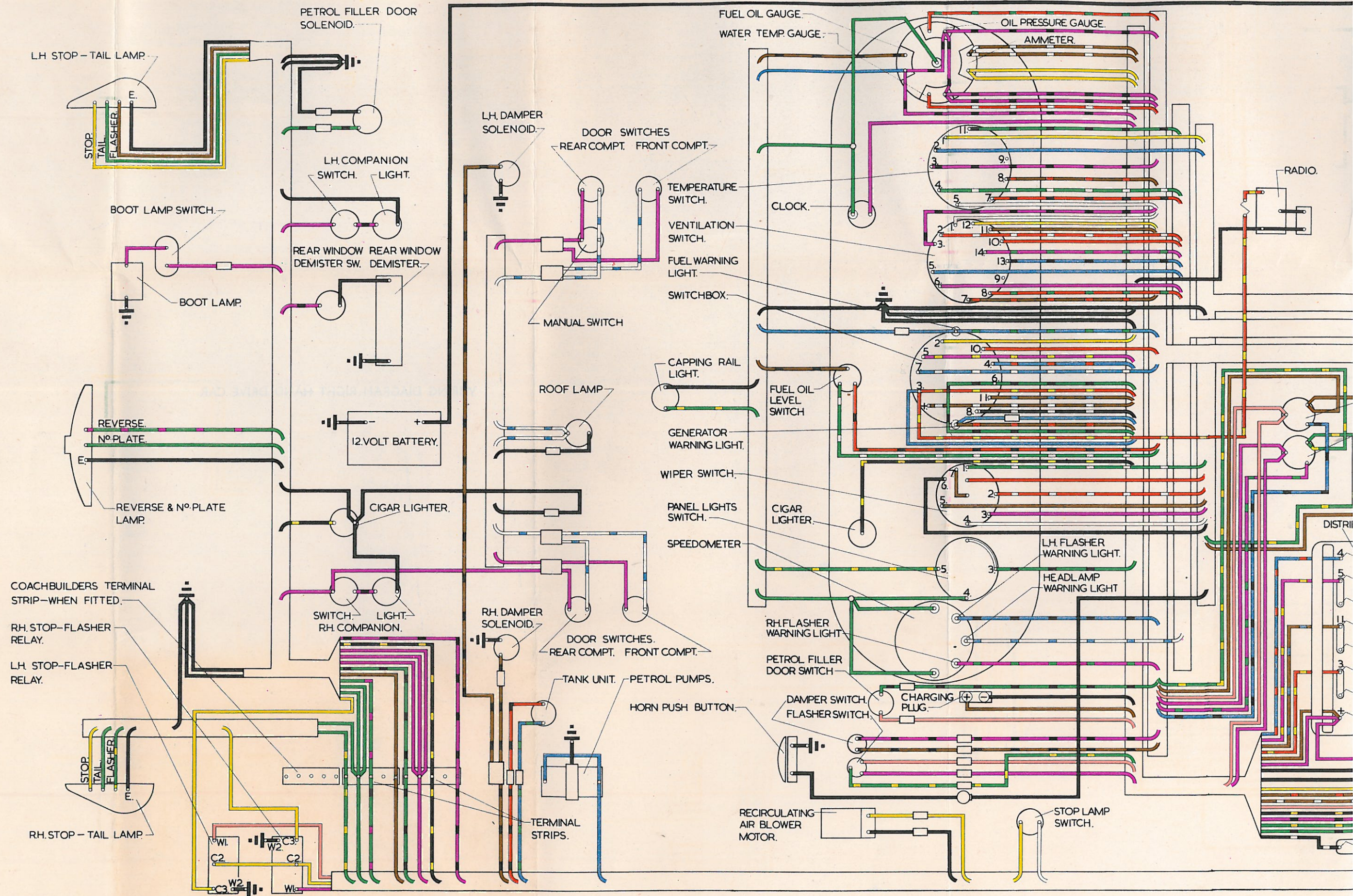
WIRING DIAGRAM
