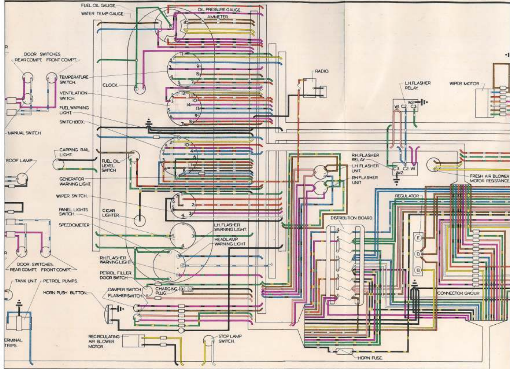
WIRING DIAGRAM RIGHT HAND DRIVE CAR
