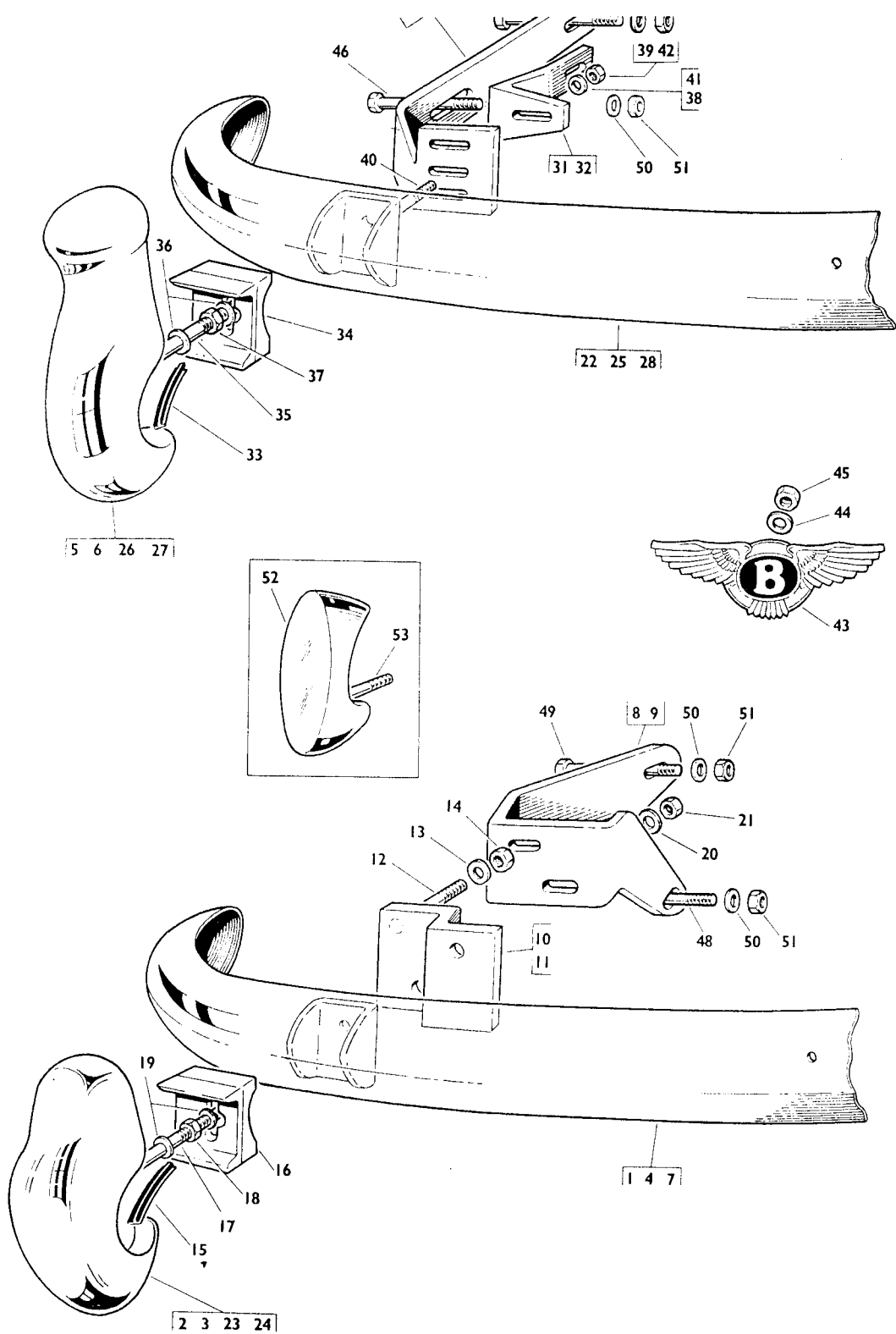
BODY- REAR BUMPER-(Park Ward And Mulliner Continental)
